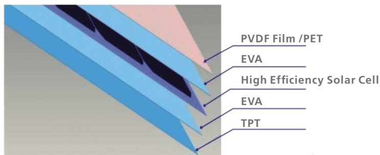
Encapsulation structure of schematic view
