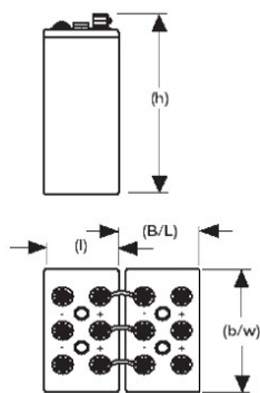
Dimension figure
