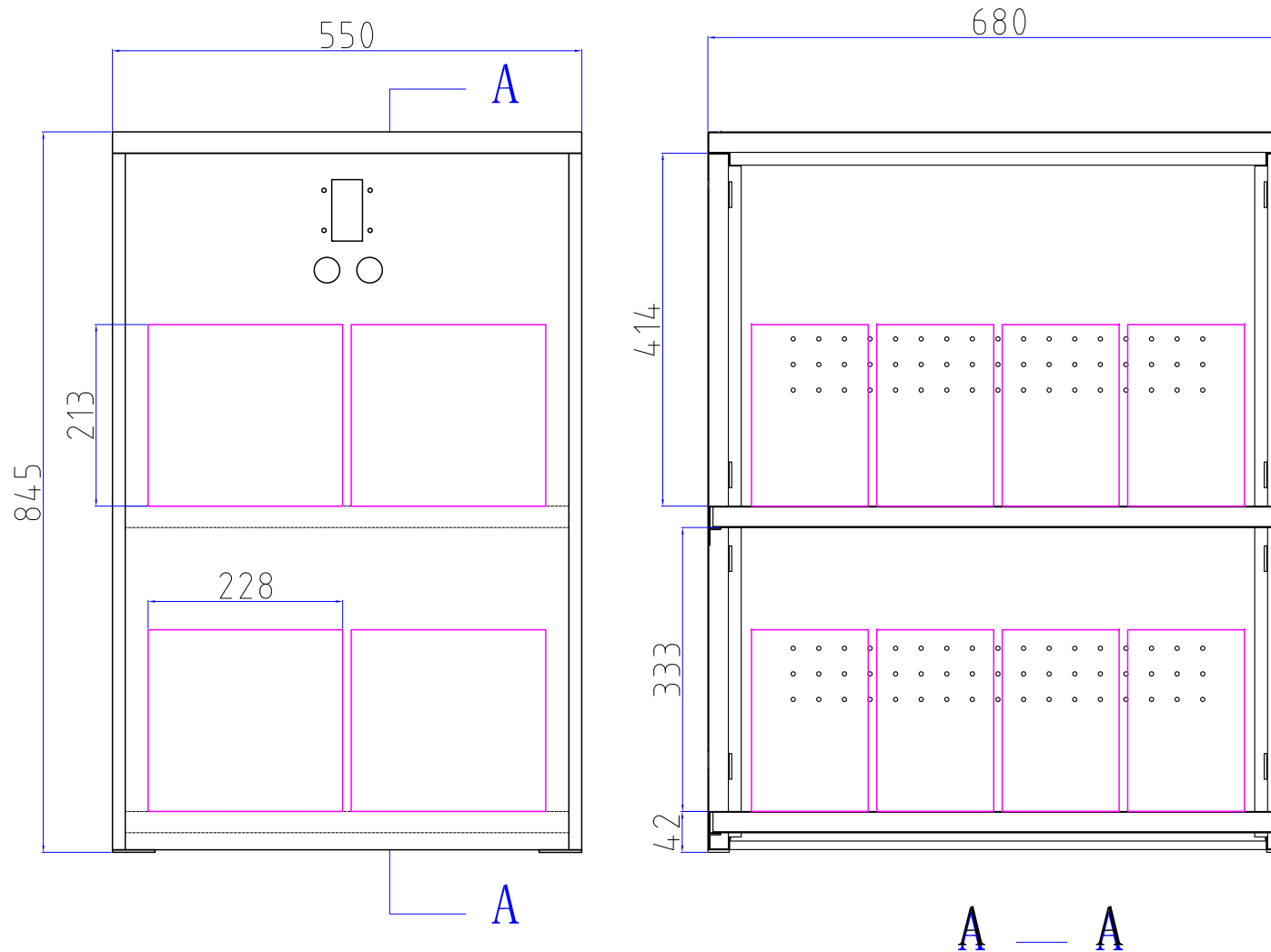
EverExceed 16pcs ST-1255 Battery Cabinet
